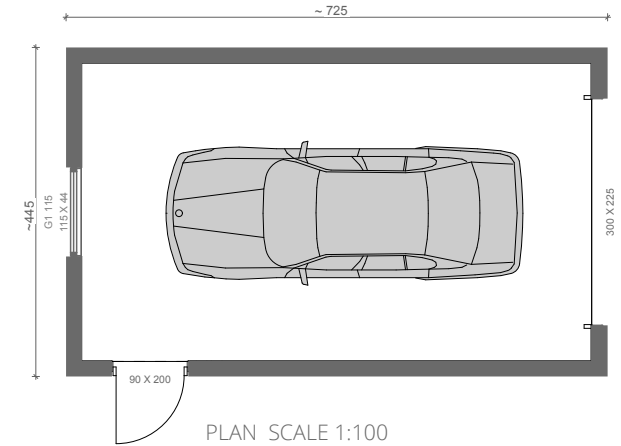
PLAN SCALE 1:100
