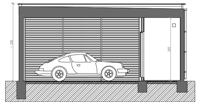
SECTION SCALE 1:100
