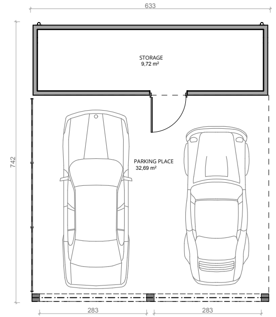
PLAN SCALE 1:100
