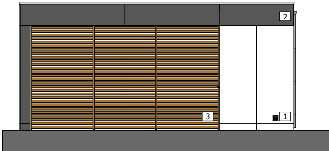
ELEVATION 3 SCALE 1:100
