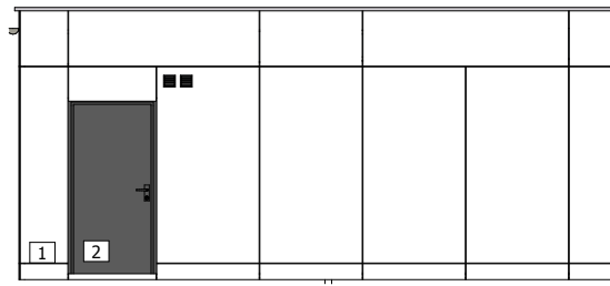
ELEVATION 4 SCALE 1:100
