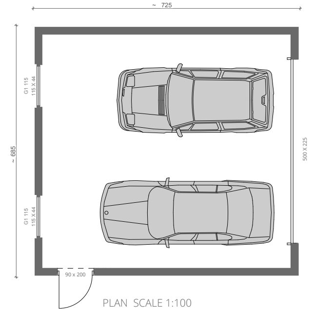
PLAN SCALE 1:100
