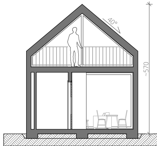
SECTION SCALE 1:100
