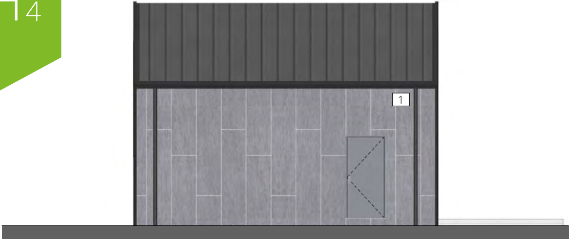
ELEVATION 1 SCALE 1:100
