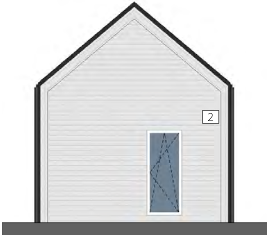
ELEVATION 4 SCALE 1:100
