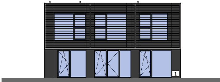
SOUTH ELEVATION SCALE 1:200
