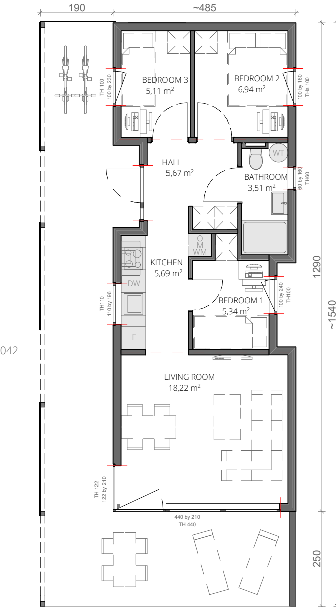
GROUND FLOOR SCALE 1:100
