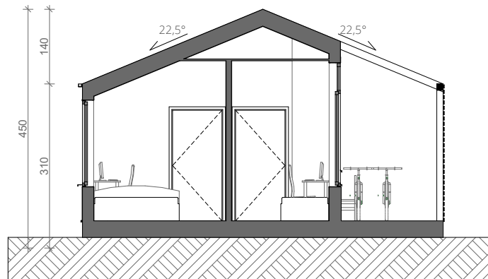
SECTION SCALE 1:100
