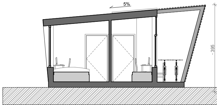
SECTION SCALE 1:100
