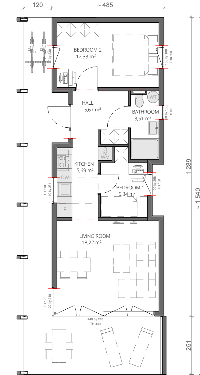
GROUND FLOOR SCALE 1:100
